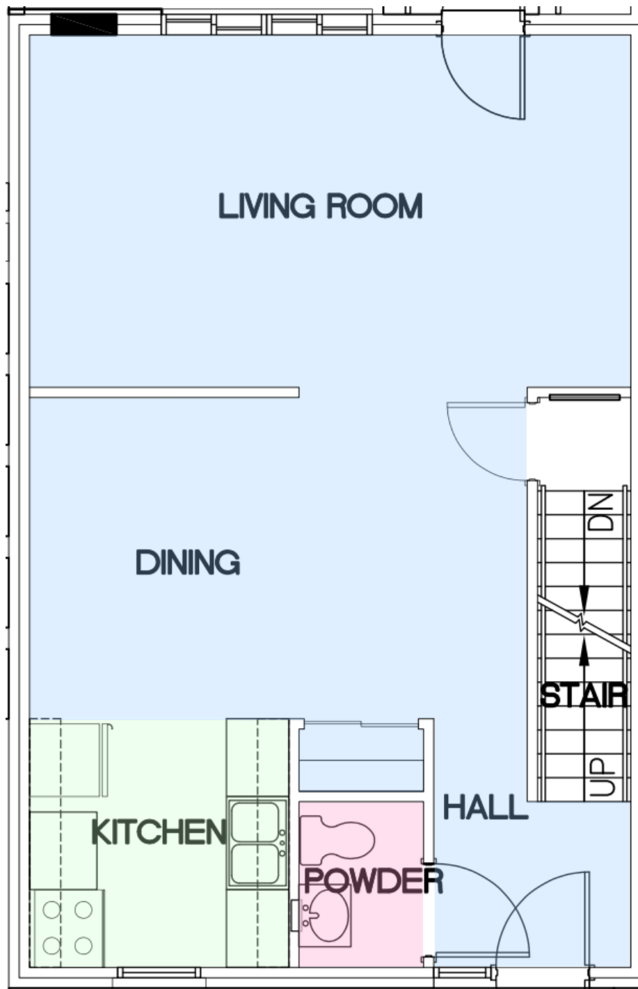
FIRST FLOOR
