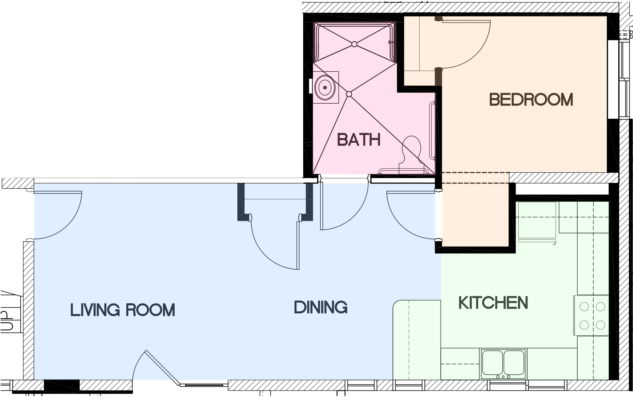
OAK PARK ONE BEDROOM ACCESSIBLE - 637 SF
